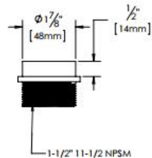
ABS or PVC Adaptor Kit Attaches to ABS or PVC Bath Wastes and includes Brass Nut and Rubber Flat Washer
