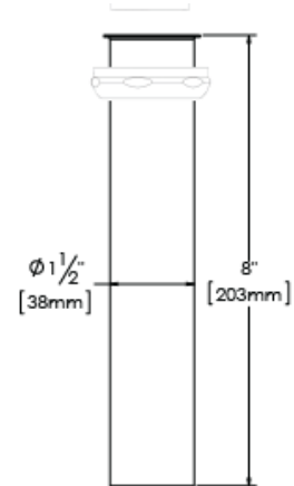
Flanged Brass Tailpiece
